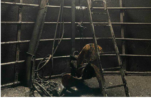
Propeller mixer blade was attached to a metal pillar inside the biodigester tank which had moved back to collide with a steel heating pipe, causing a breach
