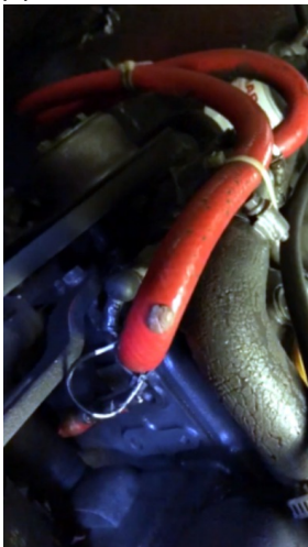
Superfast Steel was applied to the pinhole, followed by a SylWrap HD Bandage to seal the leak
